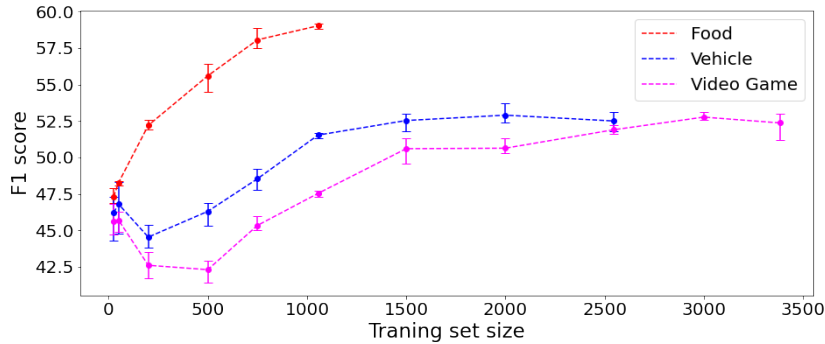
Figure 4: Summarization performance of different video categories with varied training set size
