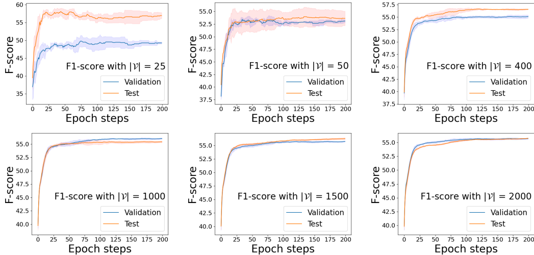
Figure 3: F1-Scores with various validation set sizes |\mathcal{V}| (Shaded area indicates \pm 1\sigma from the mean.)
